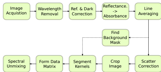
Fig. 8: Flowchart of pre-processing pipeline.
