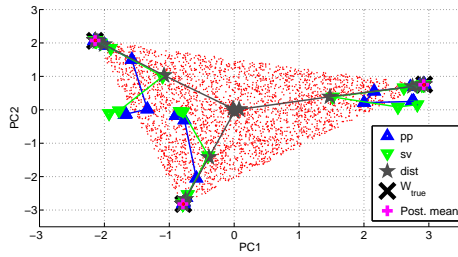
Fig. 18: Scatterplot of unmixing result with parameters ID = 3, K = 3, M = 150, \sigma^2 = 10^{-4} .
